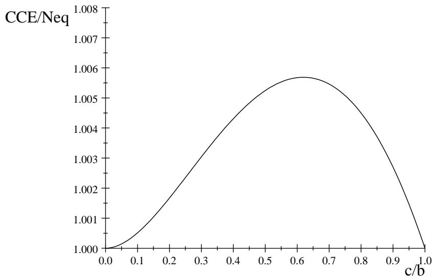
Figure 2: Mediation value in the abatement game.
