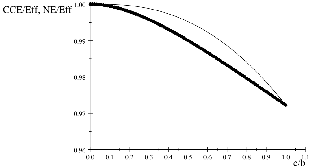
Figure 1: Enforcement value and \frac{\pi^{Neq}}{\pi^{eff}} in the abatement game
